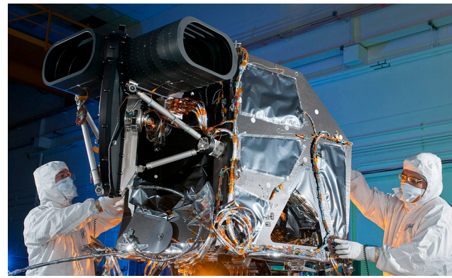
Operational Land Imager
